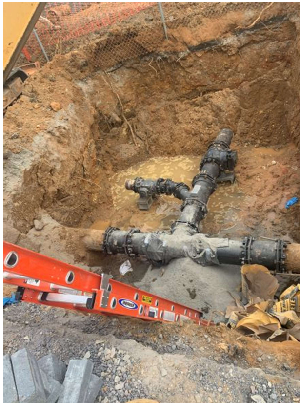
Photo 4: Bypass connection
