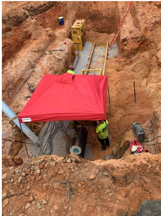
Photo 2: Bore setup
