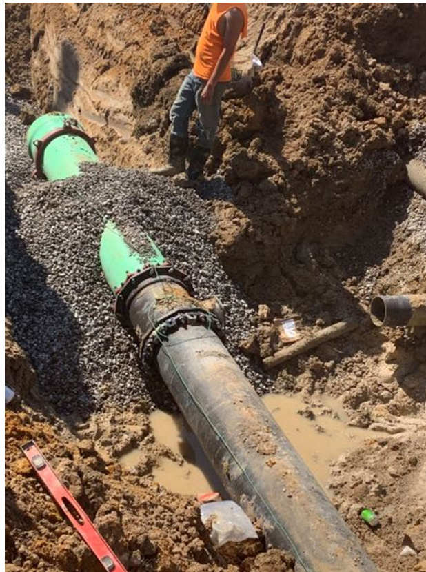
Photo 2: Line install
